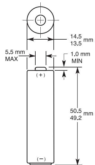
Dimensions shown are IEC standards
