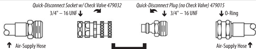
Socket and Plug Assembly 479010
